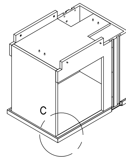
PART. C
