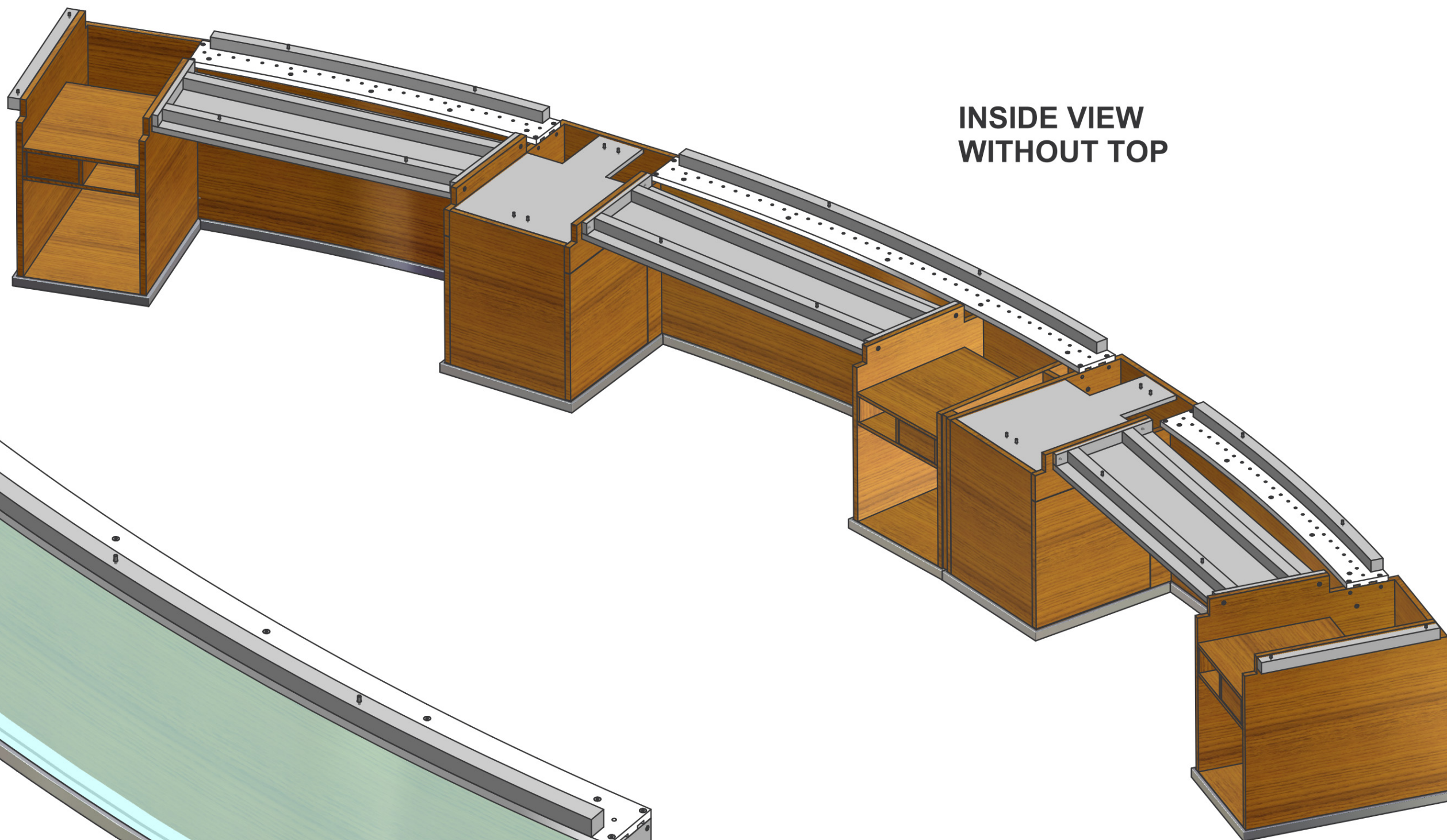
PACKING SYSTEM FOR FRONTAL PANEL
