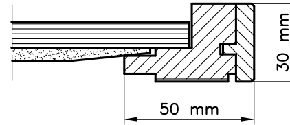
SECTION scale 1:2
